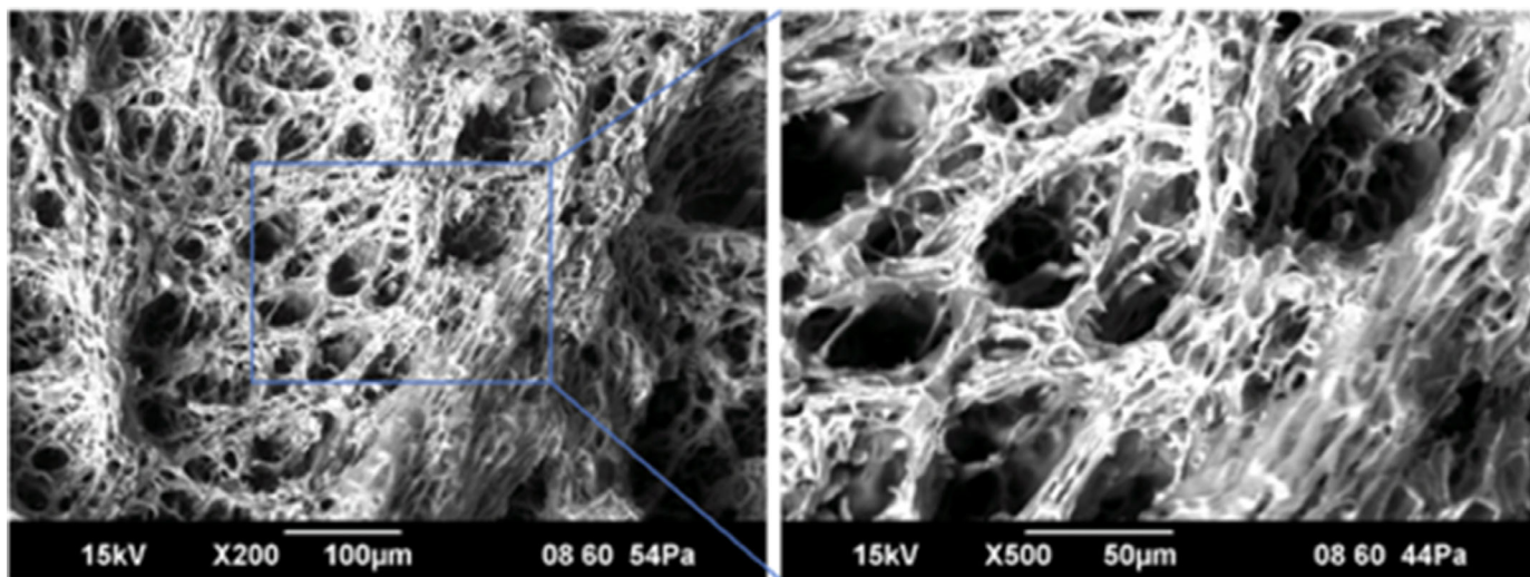
Figure 5. SEM photographs of the hydrogel structure formed by the bio-adhesive.
